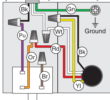
MOTOR (Wired 220V)
